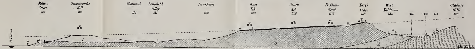
FIG. 3. SECTION ALONG THE CREST OF THE CHALK ESCARPMENT FROM LIMPSFIELD TO IGHAM.
